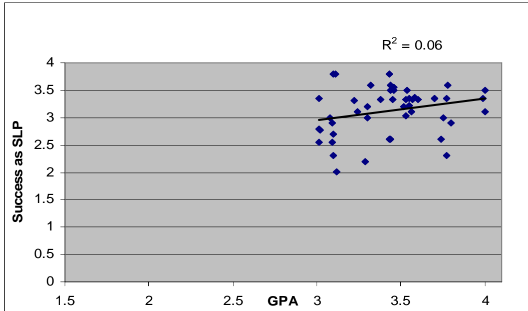
Figure 2: Correlation in the restricted range of GPA from 3.0 to 4.0, R = 0.25
