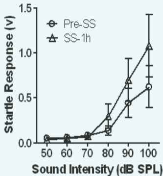
Figure 2. Effects of salicylate on the rat startle reflex response. (A) The waveform of the acoustic startle reflex induced by loud acoustic stimuli. (B) Salicylate increases the startle reflex response in an animal model.
