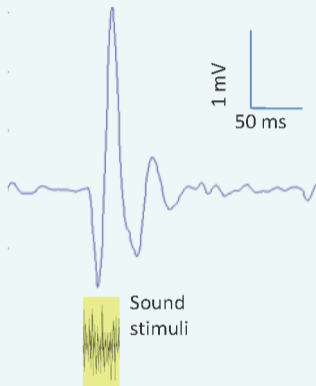
Figure 2. Effects of salicylate on the rat startle reflex response. (A) The waveform of the acoustic startle reflex induced by loud acoustic stimuli. (B) Salicylate increases the startle reflex response in an animal model.
